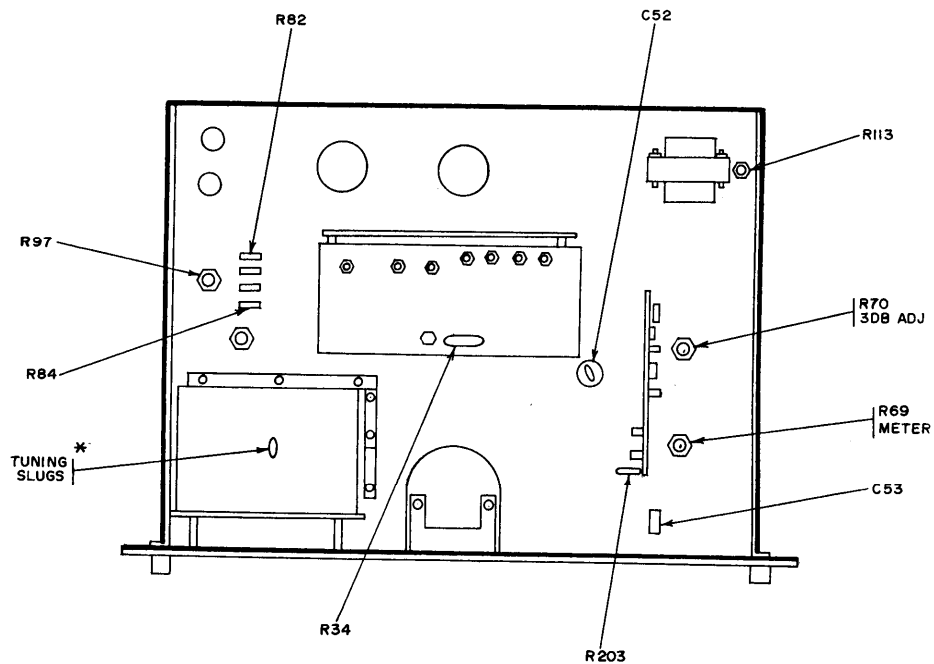
Figure 1. Test instrument, version A - top view.
